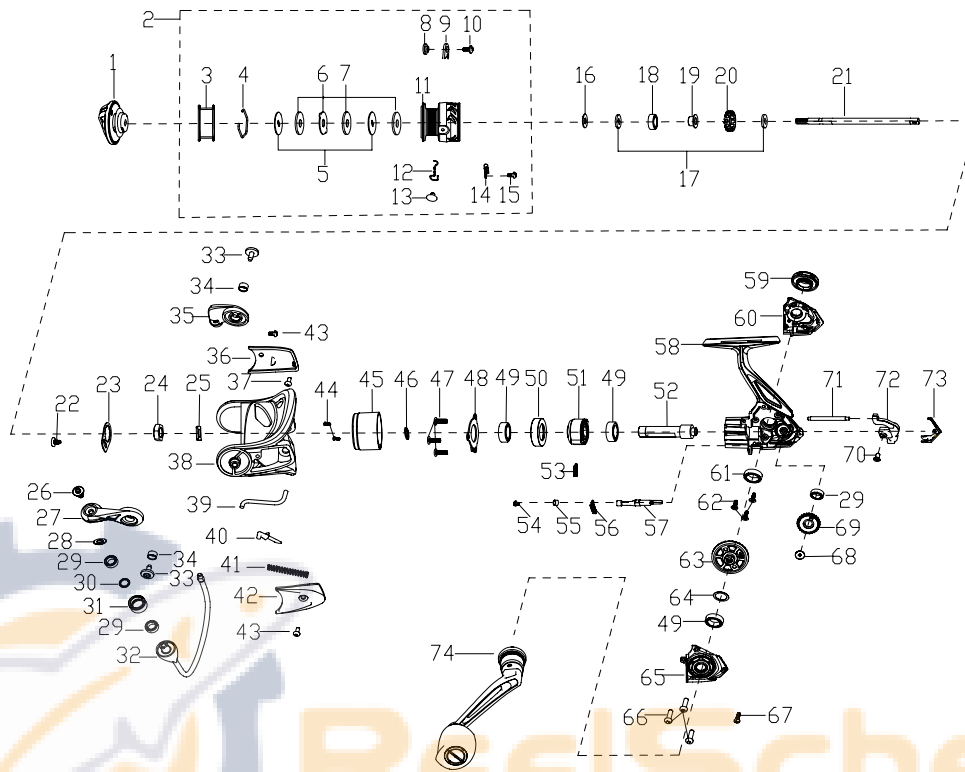
PARTS LIST OF CDB40 CS7
